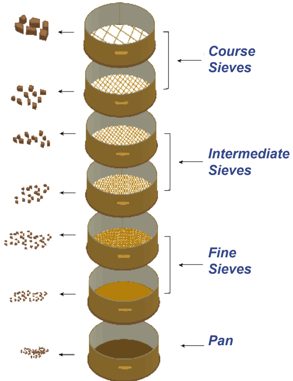
FIGURE 13: Testing gradation.
